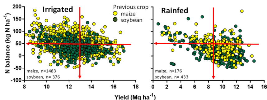
Figure 1. Nitrogen (N) balance in irrigated (left) and rainfed maize fields (right) plotted against grain yield. Each data point represents a field-year case. Data were disaggregated by previous crop: soybean (green) and maize (yellow). Horizontal arrows indicate N-balance = 50 kg N ha -1 , which was used as a threshold to identify fields with large N surplus. Vertical arrows indicate average irrigated and rainfed maize yields. Linear regression between yield and N-balance (not shown here) was significant for all water regime x previous crop combinations ( P<0.01 ).
