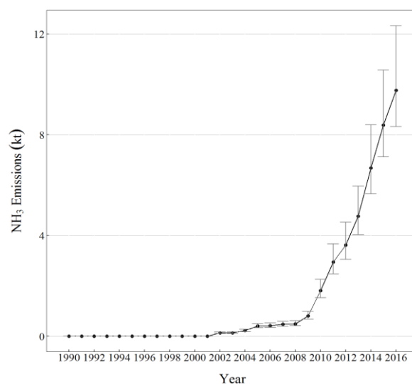
Figure 1. Estimated Emissions of Ammonia from Anaerobic Digestion in the UK. Estimated emissions of ammonia (NH 3 ) from anaerobic digestion (AD) in the United Kingdom from 1990 to 2016 in kilotons (both site-based process emissions and digestate field spreading emissions). Low and high estimates indicated by error bars (grey).
