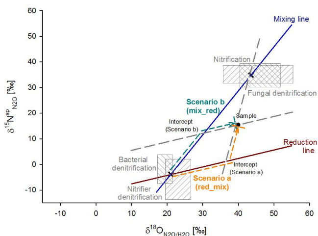
Figure 1: Isotopocule map, illustrating the simultaneous estimation of N_2O reduction and the contribution of different processes to soil-emitted N_2O
