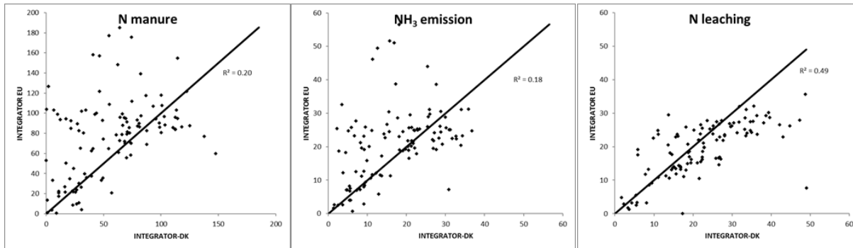
Figure 1 XY-plots for N input by animal manure, NH 3 -N emission and N leaching (in kg N ha -1 yr -1 ) as calculated by Integrator-EU and Integrator-DK for the year 2010 together with the 1:1 line and the R 2 of linear regression between the Integrator-EU and Integrator-DK results
