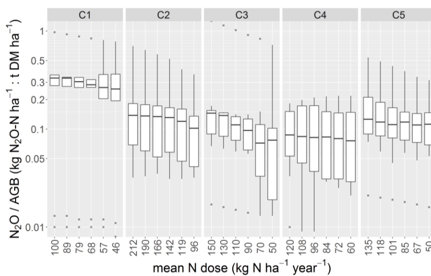
Figure 1. N 2 O to above ground biomass (AGB) ratio in the five contrasted pedoclimatic sites (C1 to C5) with N input reduction from maximum (left values on x axis) to minimum (right values). Boxplots report the response of the model ensemble. Black lines show multi-model median, boxes are 25 th and 75 th percentile, whiskers 10 th and 90 th percentile, circles indicate outliers.
