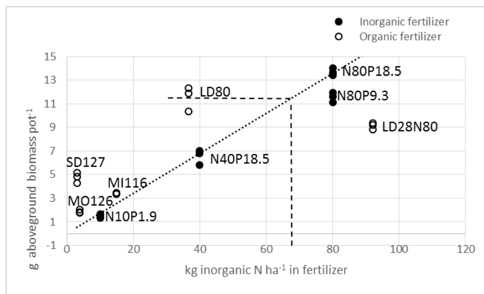
Figure 1. Yield of aboveground barley biomass in relation to the amount of inorganic N in the fertilizer. Treatments: N10P1.9 10 kg N in ammonium nitrate ha -1 + 1.9 kg of P in superphosphate ha -1 . N40P18.5 40 kg N in ammonium nitrate ha -1 + 18.5 kg of P in superphosphate ha -1 . N80P18.5 80 kg N in ammonium nitrate ha -1 + 18.5 kg of P in superphosphate ha -1 . N80P9.3 80 kg N in ammonium nitrate ha -1 + 9.3 kg of P in superphosphate ha -1 . LD80 Liquid digestate 120 kg total N ha -1 . SD127 Solid digestate 120 kg total N ha -1 . LD28N80 Liquid digestate 40 kg total N ha -1 + ammonium nitrate 80 kg N ha -1 . MO126 Sheep manure stored outdoor 120 kg total N ha -1 . MI116 Sheep manure stored indoor 120 kg total N ha -1 . The linear regression for treatments used for determining of fertilizer equivalent of N is included as a dotted line. The calculation of the fertilizer equivalent of N is illustrated with dashed lines for LD80 .
