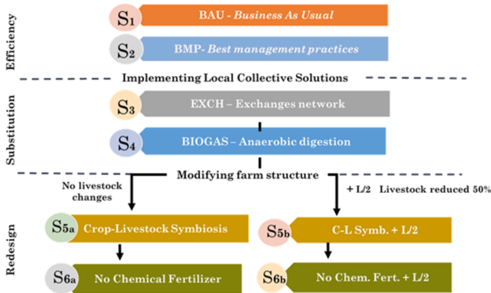
Figure 1. Scenarios explored in the Ribéracois case-study using the FAN model.
