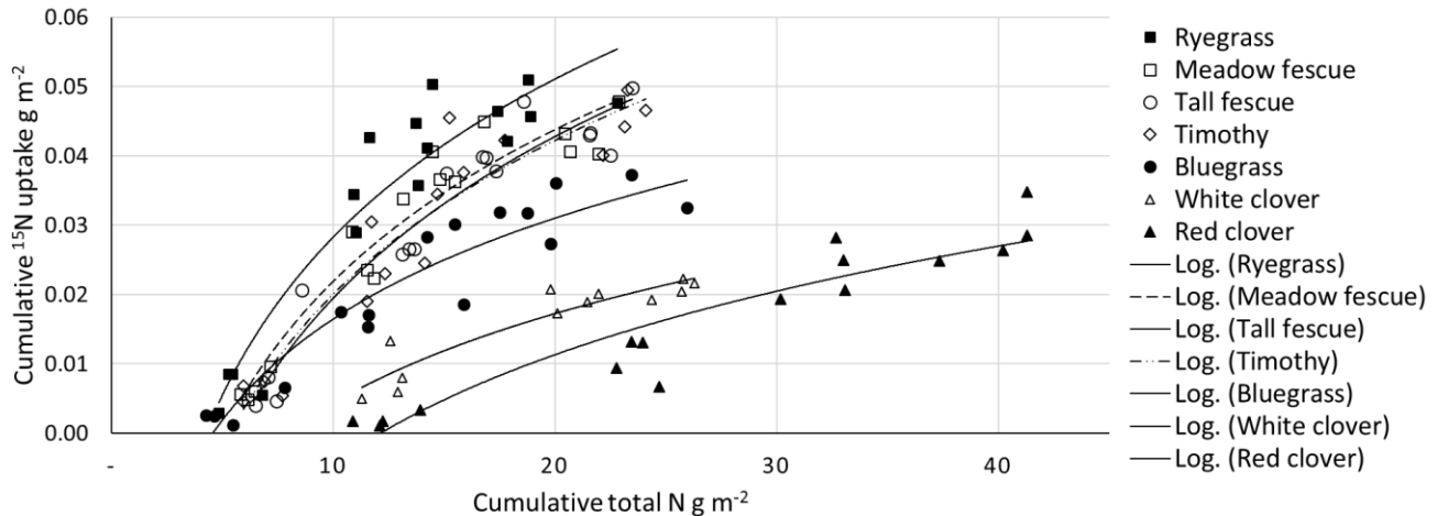
Figure 1. Cumulative 15 N uptake in four consecutive harvests, plotted versus cumulative total N content of harvested herbage. Symbols mark replicate values (4 per treatment X harvest combination). Logarithmic least square trend lines for tall fescue, meadow fescue and timothy were not significantly different from each other, whereas those for all other species were significantly higher or lower than this group ( p < 0.05 ).
