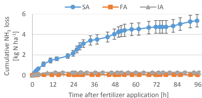
Figure 3: Cumulative NH_3 losses [ kg N ha^{-1} ] after surface application (SA), furrow application (FA) and uniform incorporation (IA) of biogas digestate during 96 hours after start of the experiment (mean values \pm stand. dev., n=3 ).
