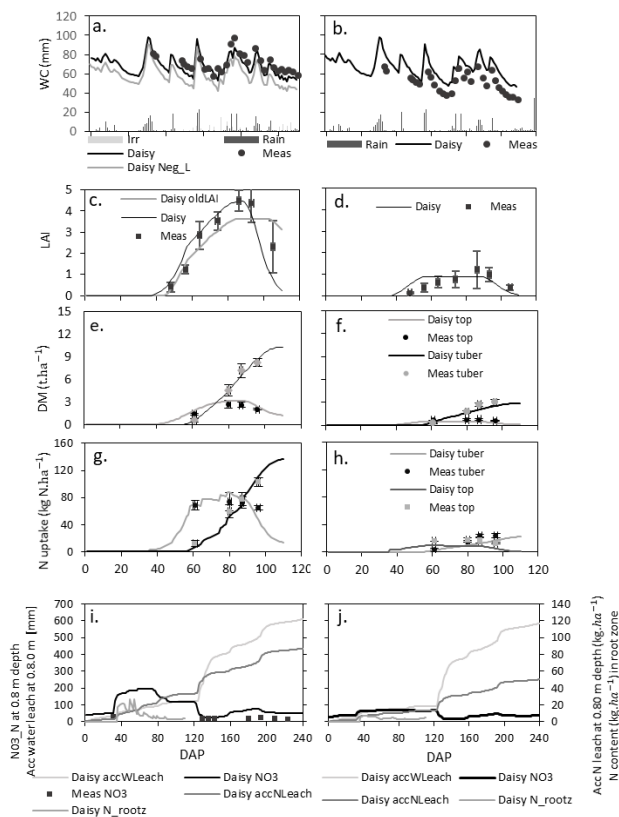
Figure 1. For I1N4 and I0N0, respectively, dynamics during the growing season of observed and simulated: a,b Soil water content. Neg_L indicates neg. I in VG-Mualem before calibration. c,d Leaf area index. OldLAI, curve before calibration. e,f Dry matter yield in top and tuber. g,h Nitrogen yield in top and tuber. Error bars in all plots indicate the standard deviation.
