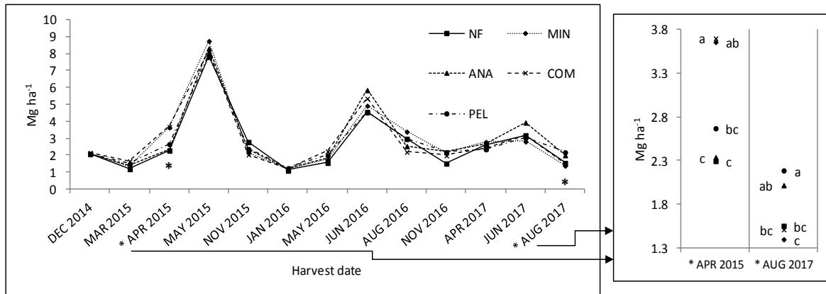
Figure 8: Pasture production (Mg dry matter ha -1 ) in all treatments under low tree density (LD). The right chart shows the production in the two harvests with significant differences. NF: no fertilisation, MIN: mineral; ANA: anaerobic sludge; COM: composted sludge and PEL: pelletised sludge. * indicates that in that harvest there were significant differences between treatments. Different letters indicate significant differences between fertiliser treatments in each harvest.
