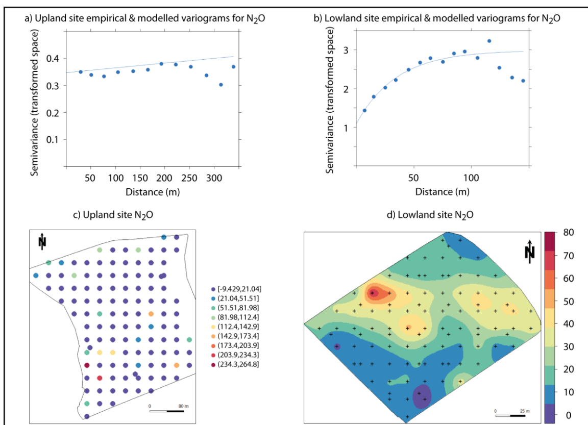
Figure 1. Empirical and modelled variograms: a) upland and b) lowland, and maps: c) upland and d) lowland of N 2 O.
