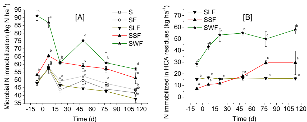
Figure 1. [A] Microbial N immobilization ( \text{kg N ha}^{-1} ), [B] physical and/or chemical N immobilization by the remaining HCA residues in \text{kg N ha}^{-1} in soil of the control treatment (S, open quadrat; Fig. 1-A) without any fertilizer or HCA, the fertilizer control treatment (SF, open circle; Fig. 1-A) with mineral N fertilizer, and the HCA treatments with mineral N fertilizer plus lignin (SLF, solid triangle downwards), spruce sawdust (SSF, solid triangle upwards), or wheat straw (SWF, solid star symbol). Incubation time d = 0 divides the x-axis into a period before (-7 DBF) and after (7, 21, 49, 77, and 113 DAF) mineral N fertilization. Standard deviations of mean values ( n=3 ) are displayed. Statistically significant differences between treatments at a certain incubation time point are depicted by different lowercase letters next to the symbols ( p < 0.05 ).
