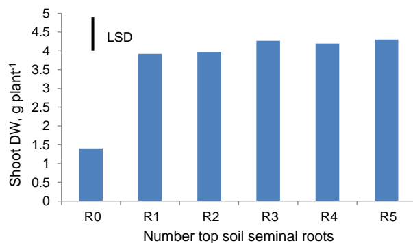
Figure 1. Spring wheat dry weight across treatments of 0 to 5 seminal roots in the topsoil
