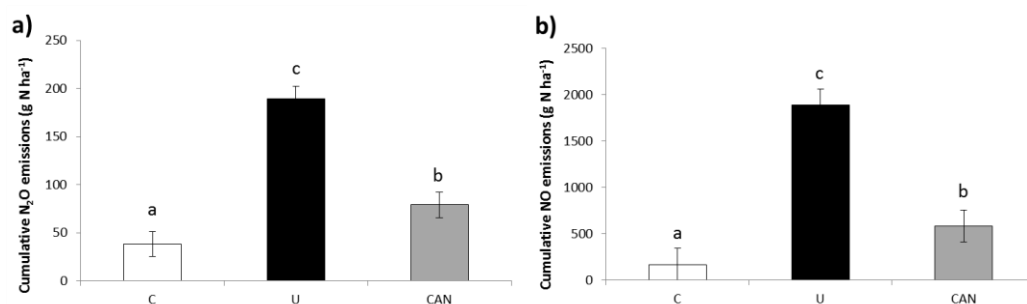
Figure 1. Cumulative N 2 O (a) and NO (b) emissions from fertilization to harvesting. Different letters within columns indicate significant differences by applying the Least Significant Difference (LSD) test at P < 0.05 . Vertical bars indicate standard errors.
