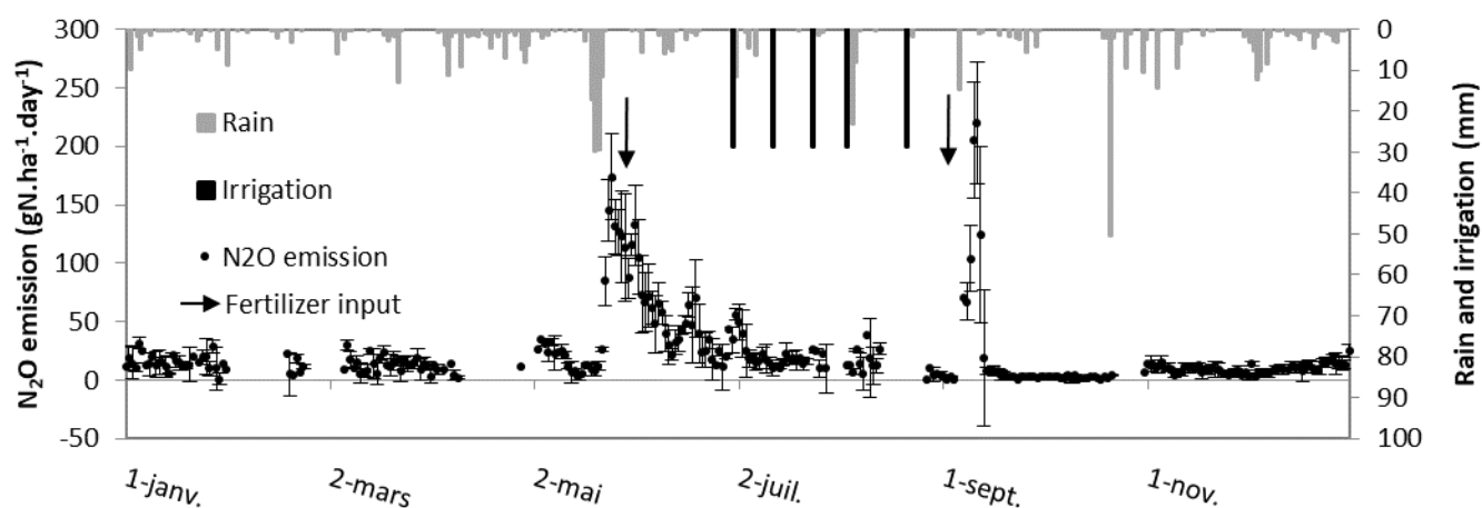
Figure 5. Daily dynamic of N 2 O emissions from a maize crop at FR-Lam site during the year 2012: sowing on 27 April, harvest on 23 August, fertilizer: 110 kg N.ha -1 on 30 May and 120 kg N.ha -1 as manure on 4 September.
