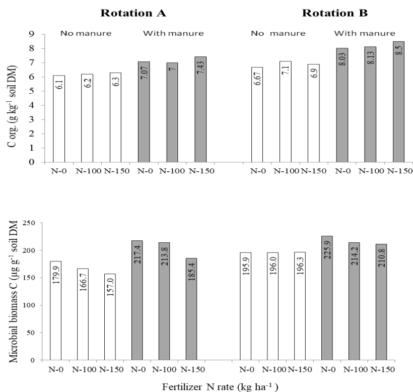
Figure 1. Organic C and microbial biomass C contents in soil as influenced by crop rotation (I), manure application (II) and mineral N rate (III) in a long-term field experiment. LSD(P \leq 0.05) : for C org.: I = 0.52, II = 0.65, III = 0.23, interactions – not significant; for microbial biomass C: I = 11.5, II = 10.1, III = 11.2, interactions: not significant
