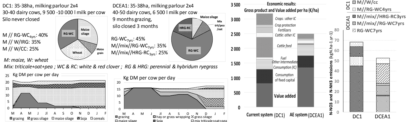
Figure 1: Comparison of DC1 and DCEA1 on technical, economical and N emissions (Syst'N results, hatched areas = N-NO 3 leached, dotted areas = N-NH 3 volatilised)
